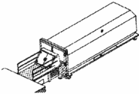
Typical dock loading bulkhead enclosure with safety rails, gate and diamond plate decking
