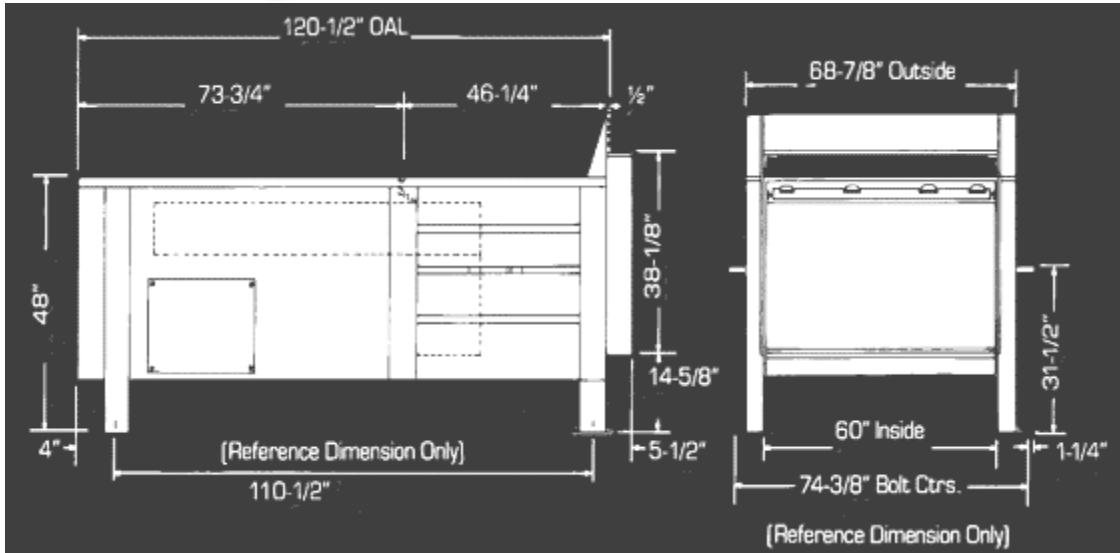
DIMENSIONS FOR 2 CUBIC YARD STATIONARY COMPACTOR UNIT (Shown without accessories)
