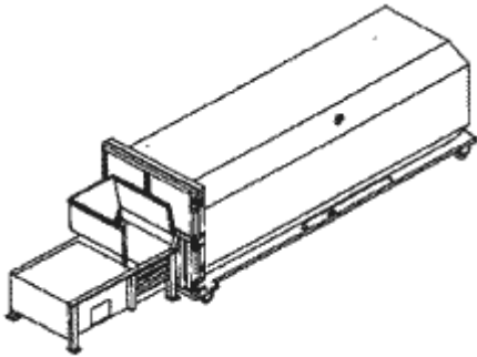
Typical side-loading security-chute with inside U/L security fire door
